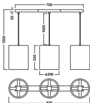
DECOR CARDBOARD CYLINDER PEND 3XE27
