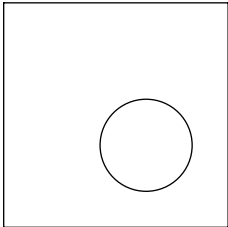
NODE SQUARE 02 BIG WALL LAMP, W37 x H37 x D20 cm SMALL GLASS GLOBE, Ø16 cm ART NO. 83010100nn, 83010101nn
