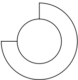
NODE CIRCLE 02 SMALL WALL LAMP, W28 x H28 x D20 cm SMALL GLASS GLOBE, Ø16 cm ART NO. 83003100nn, 83003101nn
