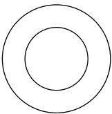
NODE CIRCLE 03 SMALL WALL LAMP, W28 x H28 x D20 cm SMALL GLASS GLOBE, Ø16 cm ART NO. 83005100nn, 83005101nn
