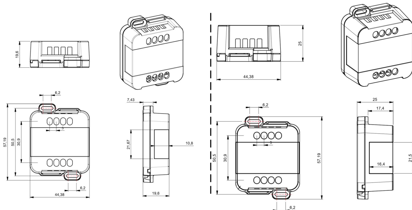
DLM1224-1CV-BUS Variant
