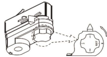
4-wires adaptor
