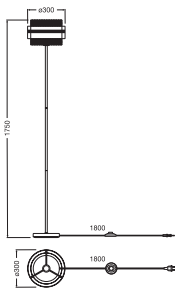
DECOR HORNET FLOOR 1XE27
