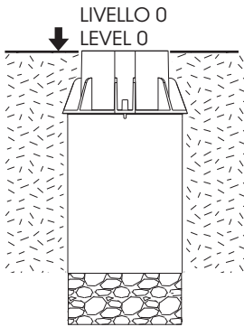
Cassaforma a filo pavimento finito Recessed box to be flush with the installation surface
