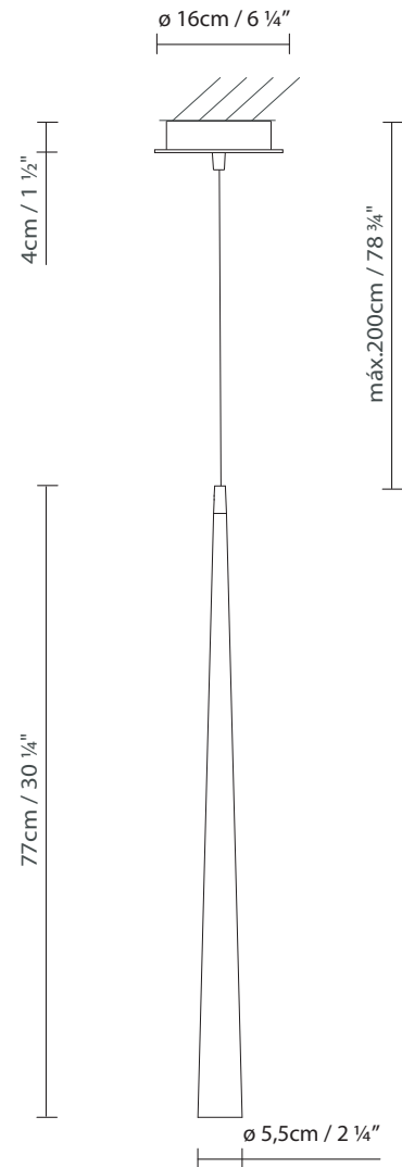
MICRO S75
