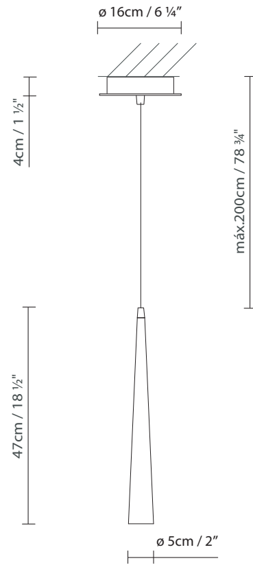
MICRO S50
