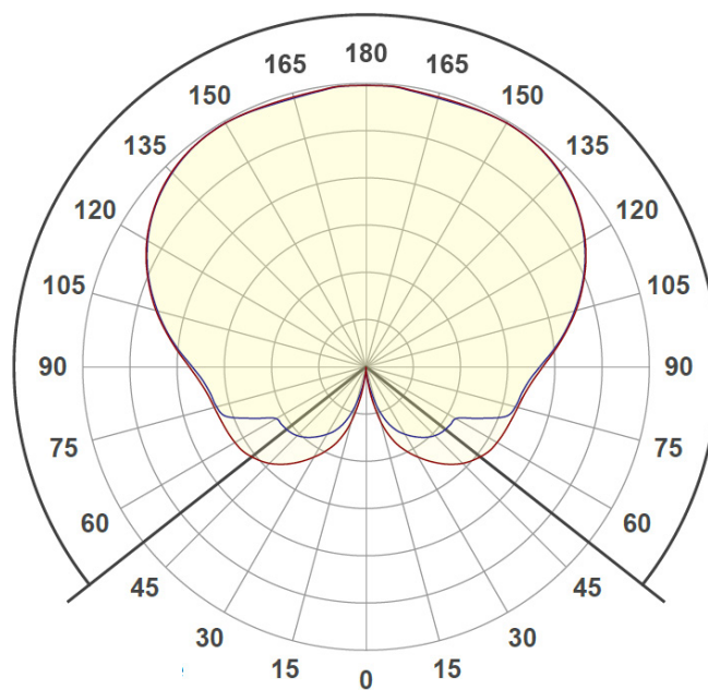
Beam angle: 256,5° Intensity distribution - Polar
