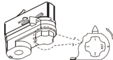
4-wires adaptor
