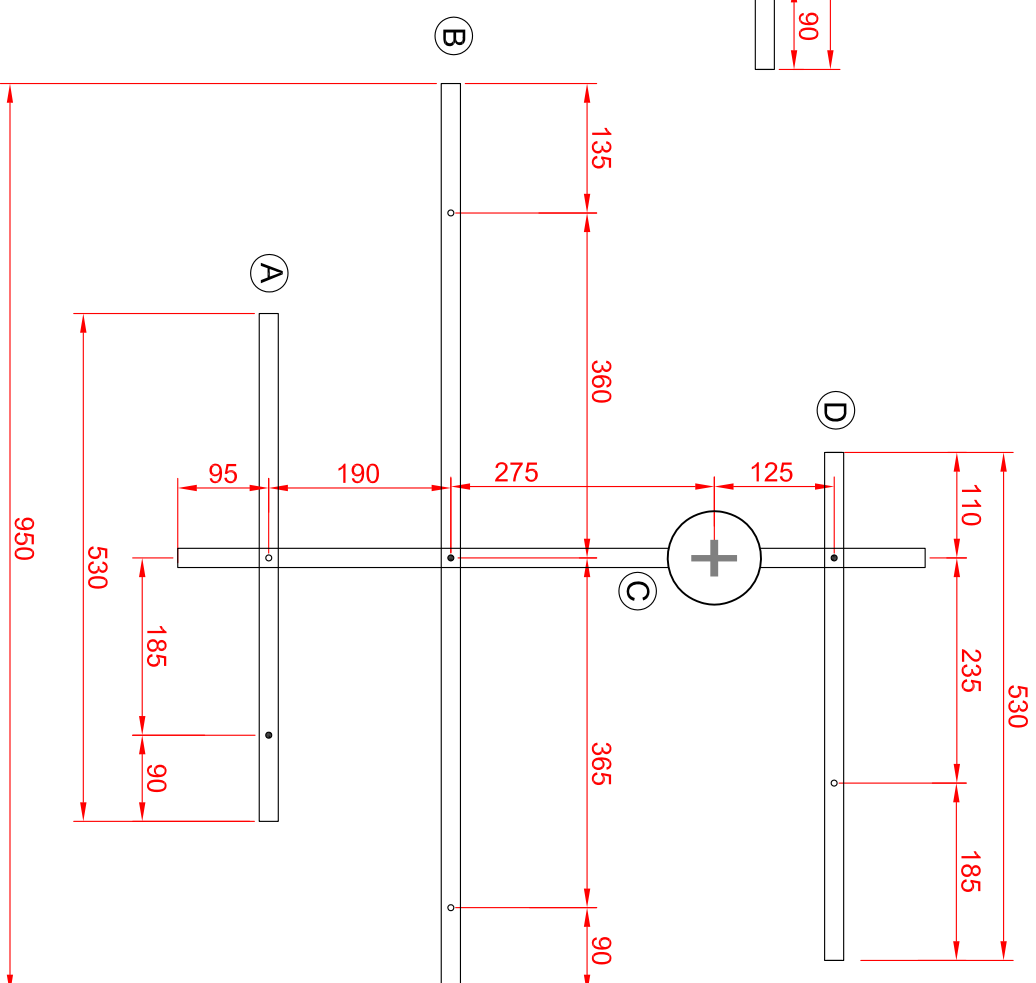
1744.178 Wall mounting-hole Distribution diagram
