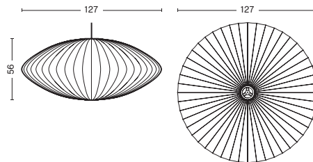
SAUCER | X-LARGE DIAMETER 127 CM | 50" HEIGHT 56 CM | 22.05"
