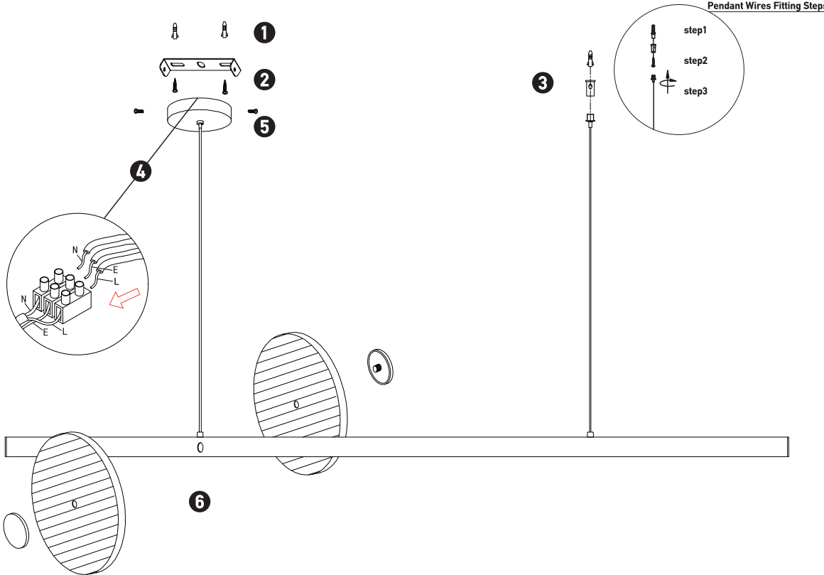
Pendant Wires Fitting Steps
