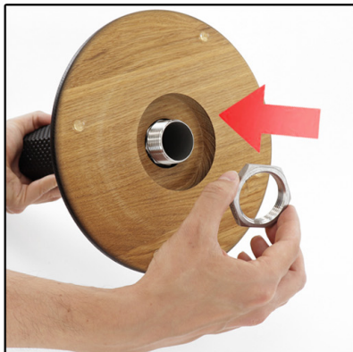
5 Metallring schrauben Screw ring
