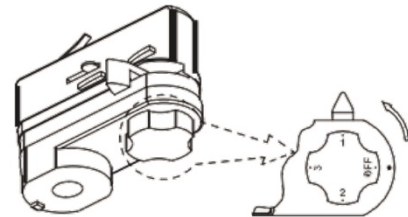
4-wires adaptor
