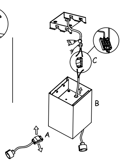
KIT GU10
